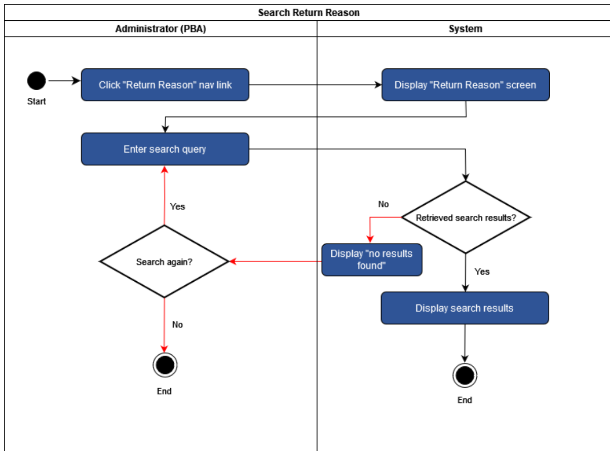
Figure 28 - Search Return Reason use case 4.14
