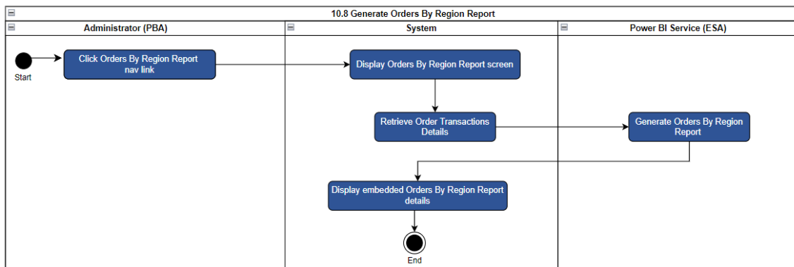
Figure 114 - Generate Order (by Region) Report use case 10.8
