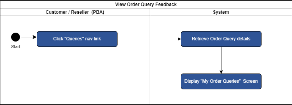
Figure 63 -View Order Query Feedback use case 6.6
