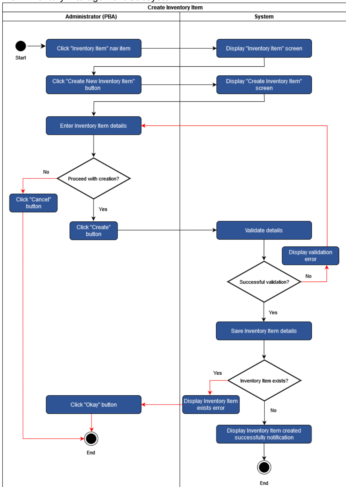
Figure 69 – Create Inventory Item use case 8.1
