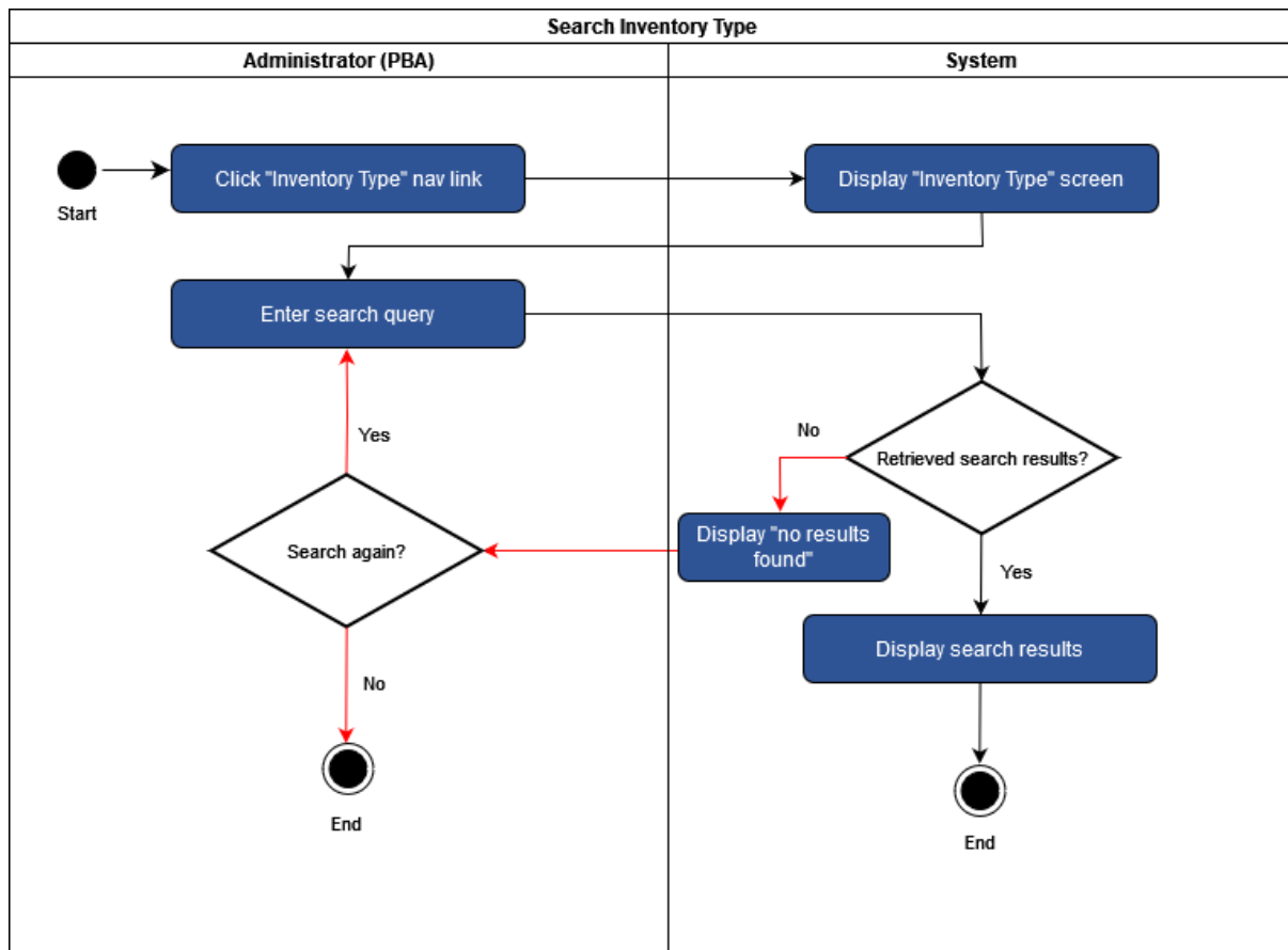
Figure 74 – Search Inventory Type use case 8.6
