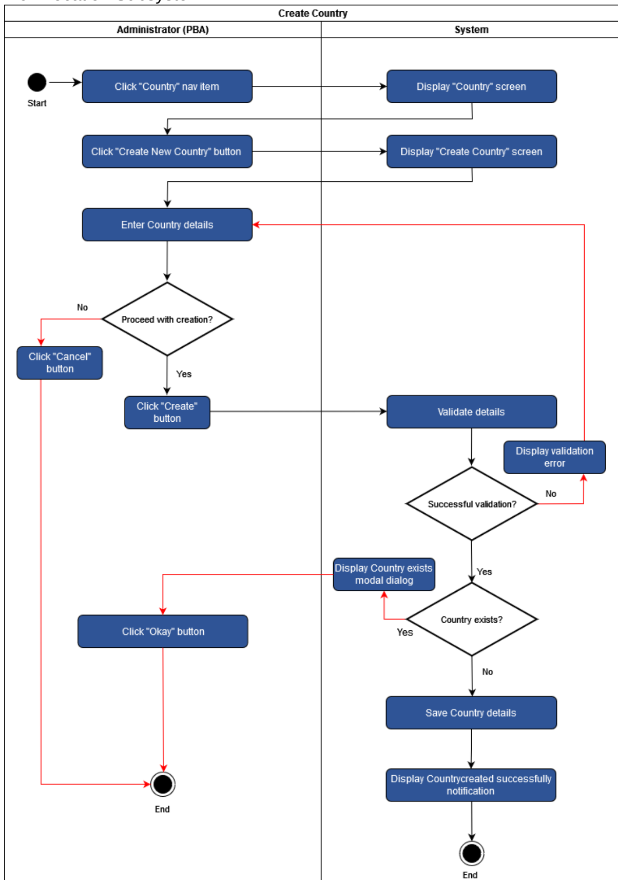
Figure 91 – Create Country use case 9.1
