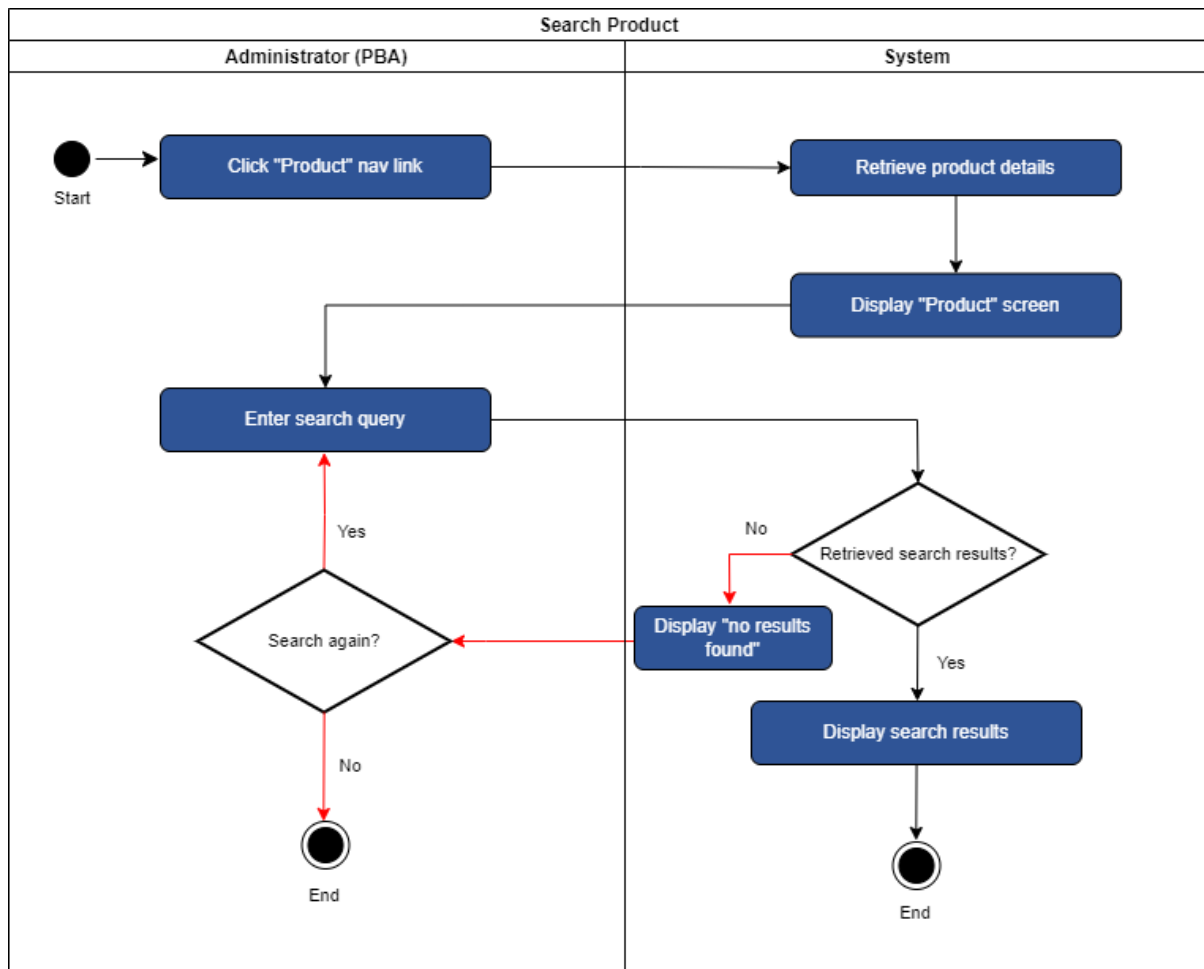
Figure 16 - Search Product use case 4.2
