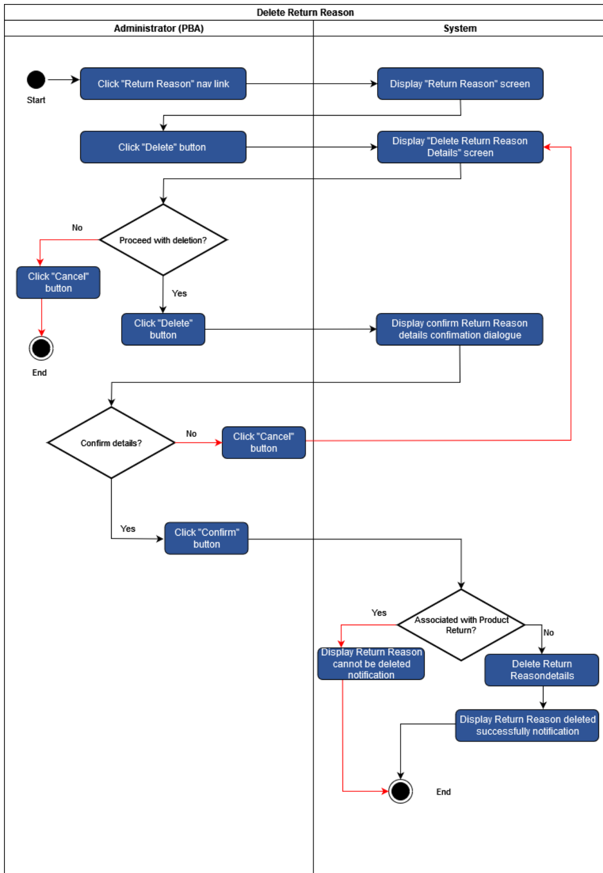
Figure 30 - Delete Return Reason use case 4.16
