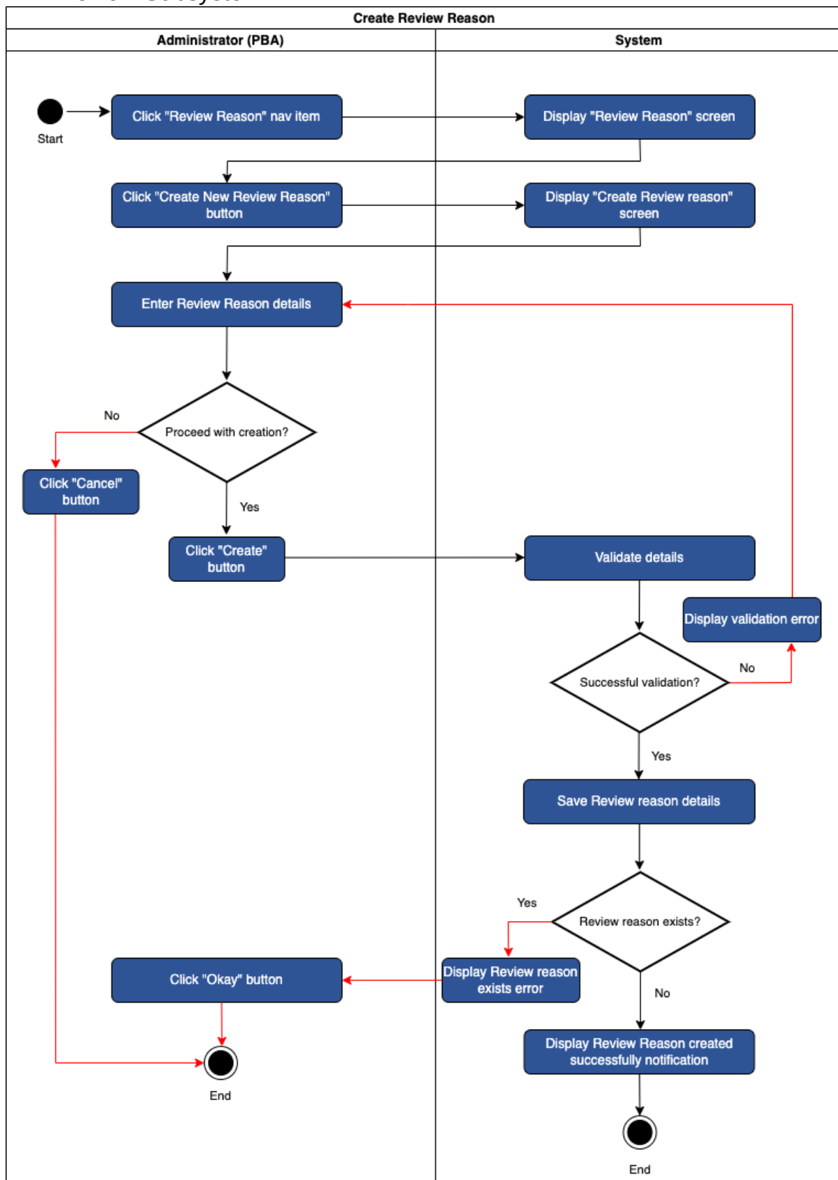
Figure 64 - Create Review Reason use case 7.1
