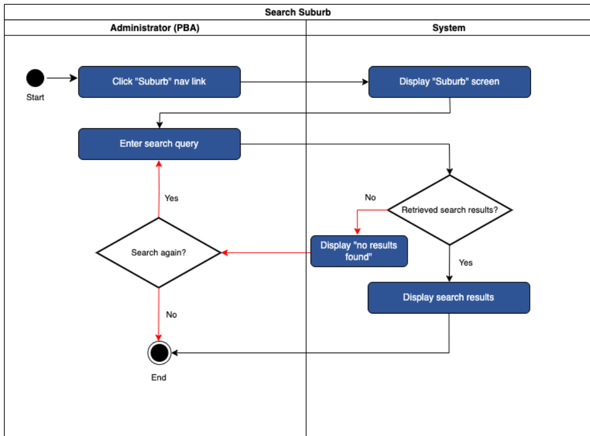
Figure 104 –Search Suburb use case 9.14
