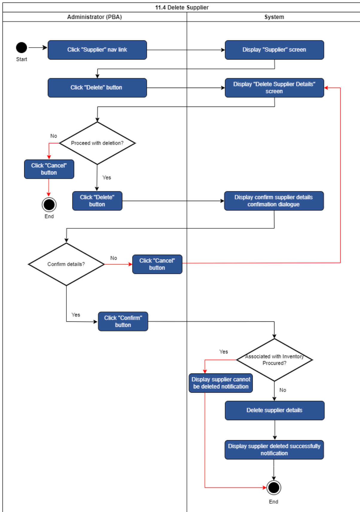
Figure 121 – Delete Supplier use case 11.4
