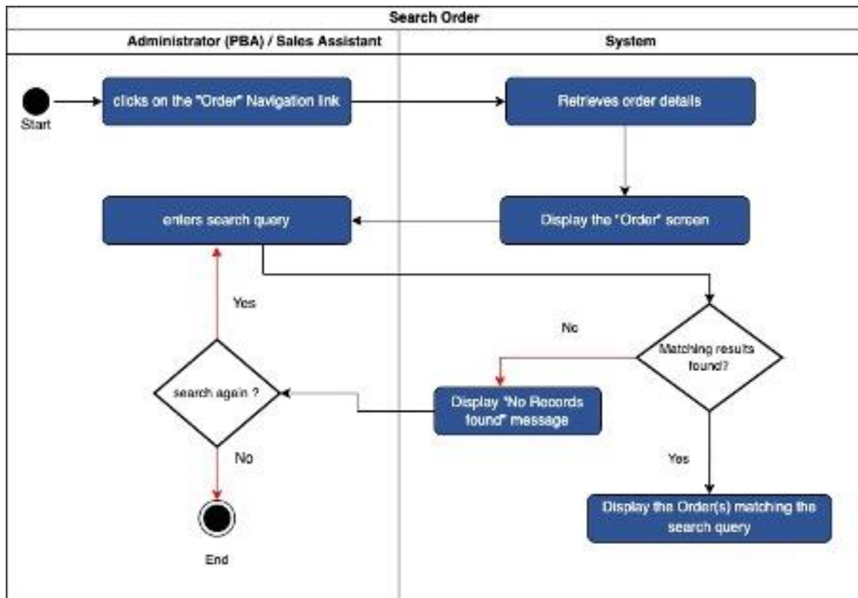
Figure 40– Search Order use case 5.8
