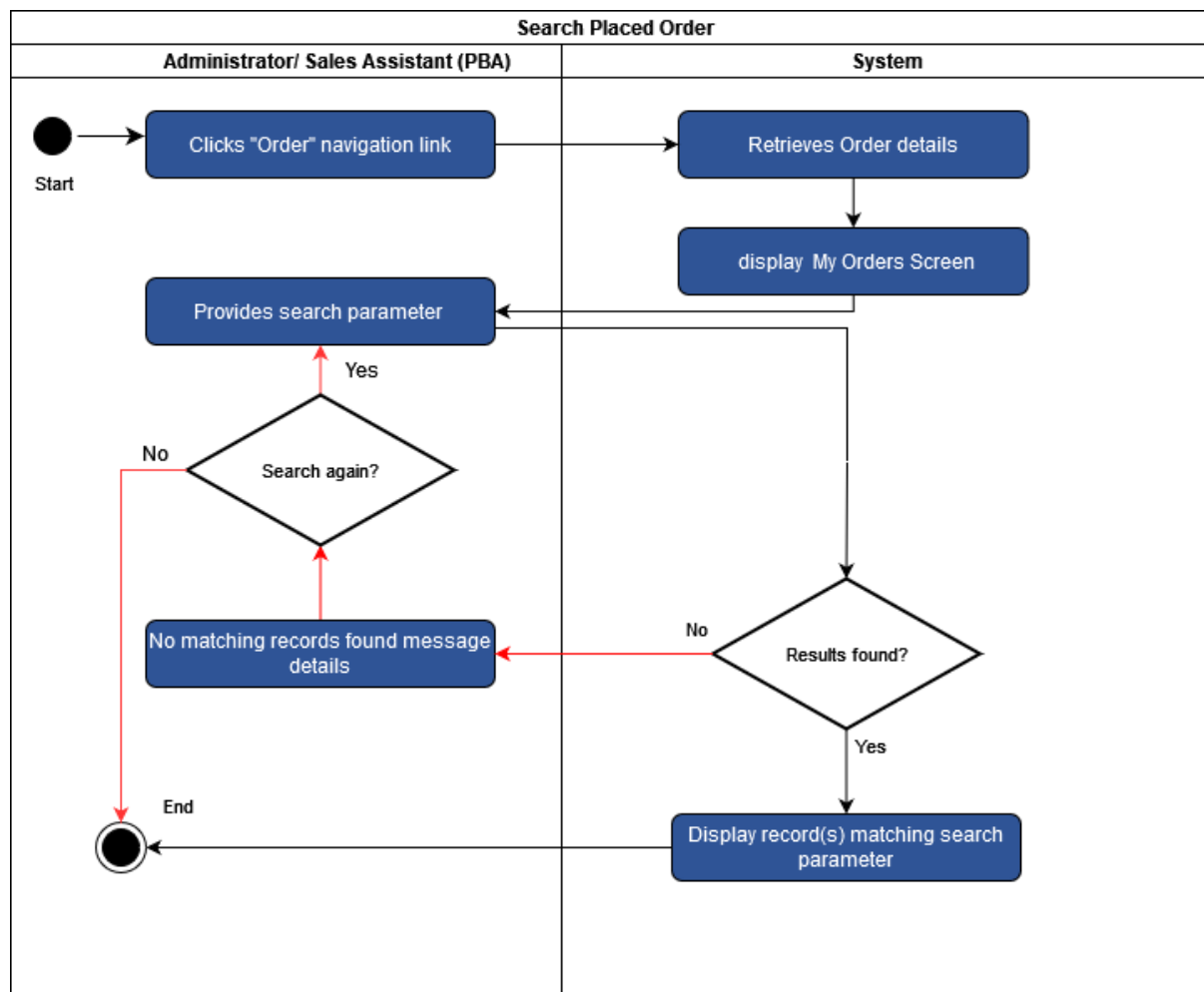
Figure 47 – Search Placed Order use case 5.15
