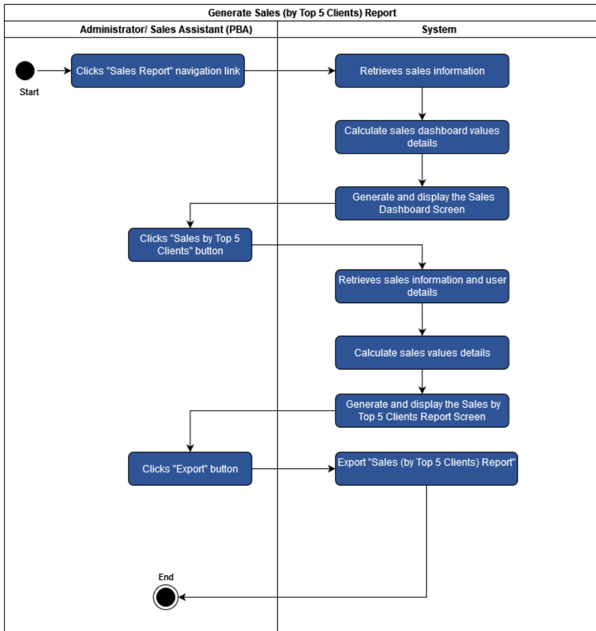
Figure 108 - Generate Sales (by Top 5 Clients) Report use case 10.2
