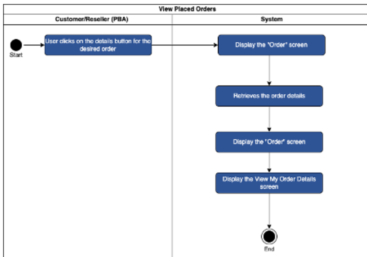
Figure 48 – View Placed Order use case 5.16
