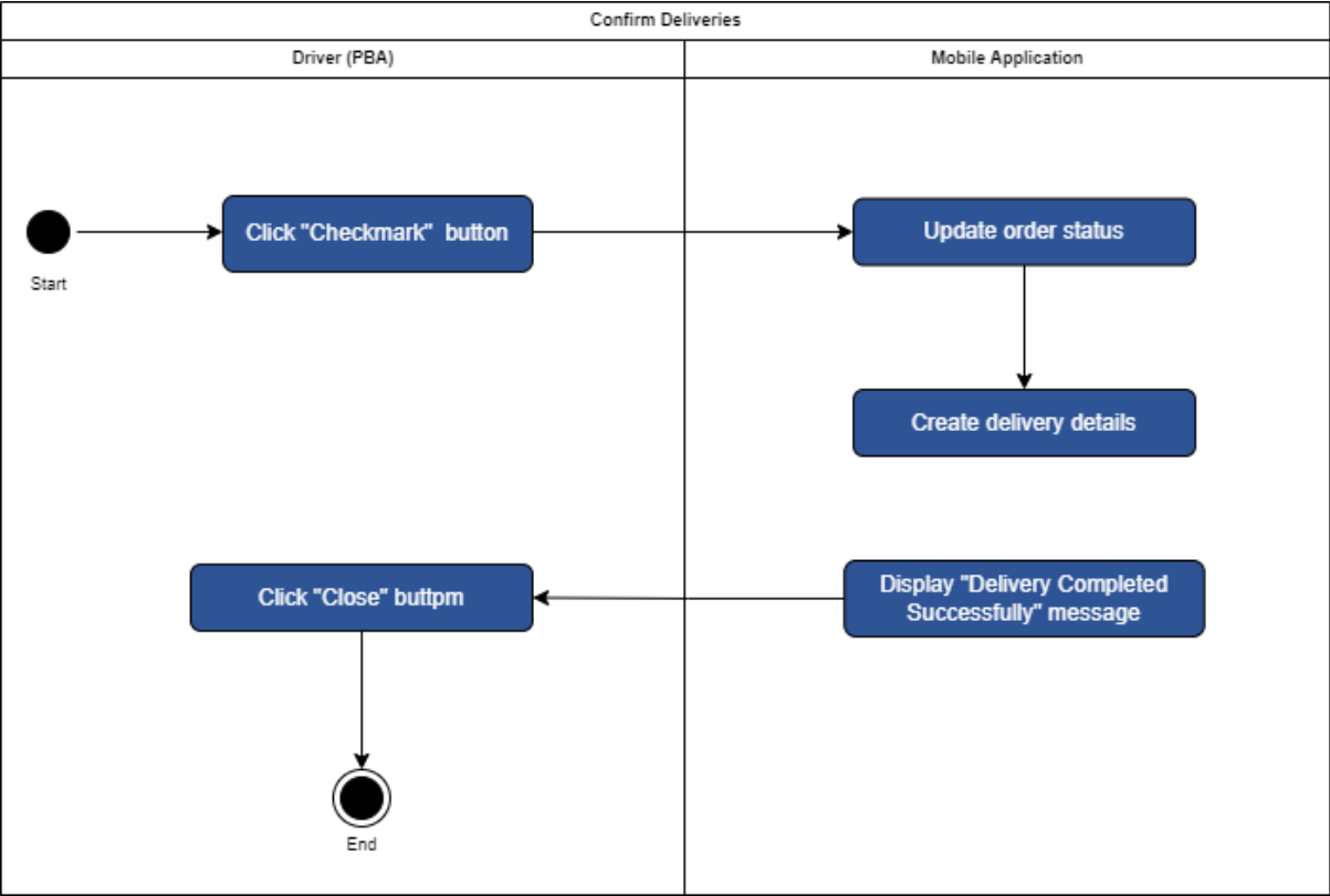
Figure 125 – Confirm Delivery use case 12.3
