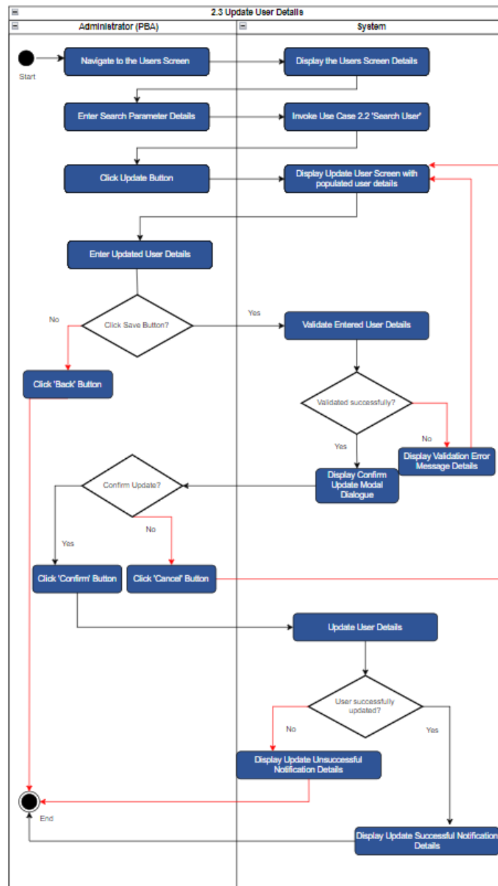
Figure 11- Update User Details use case 2.3
