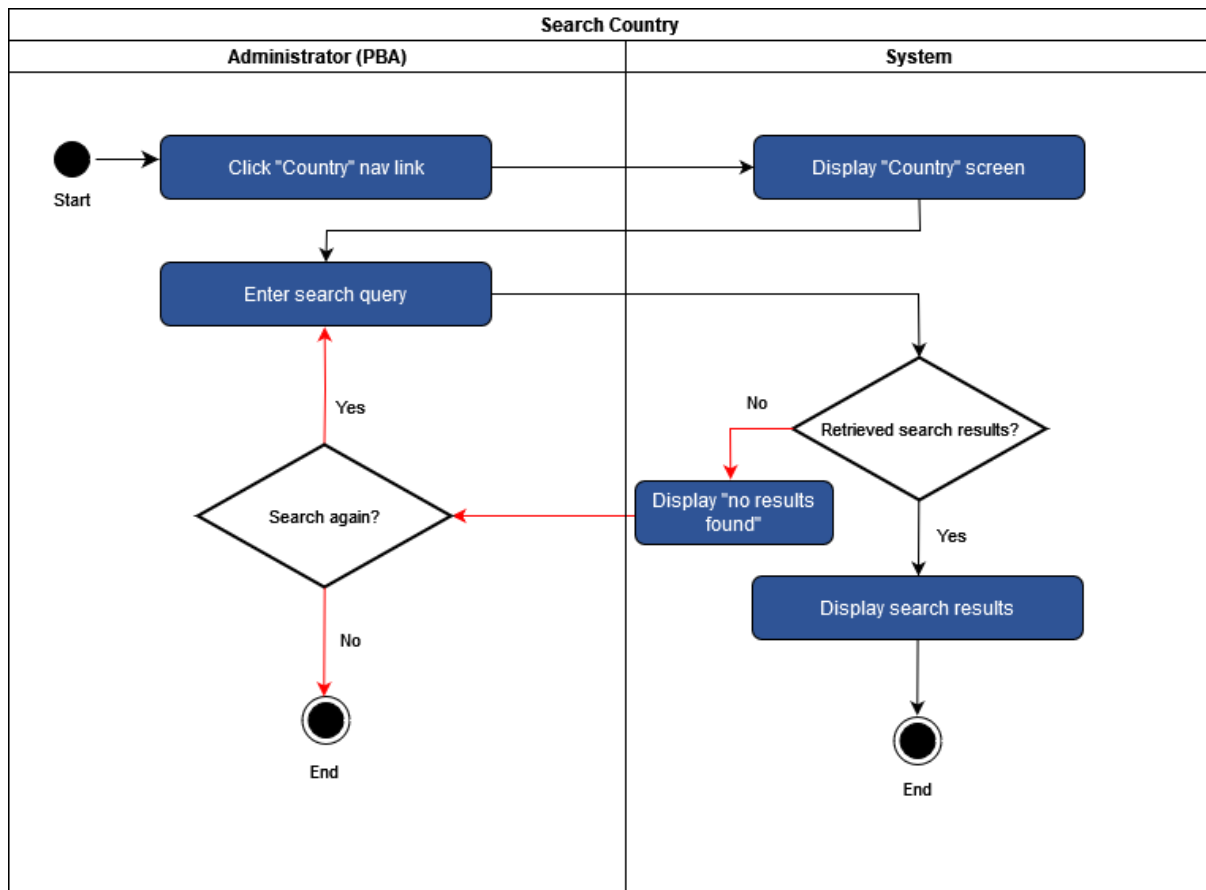
Figure 92 – Search Country use case 9.2
